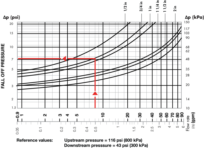
Graph 2 (Pressure drop)
